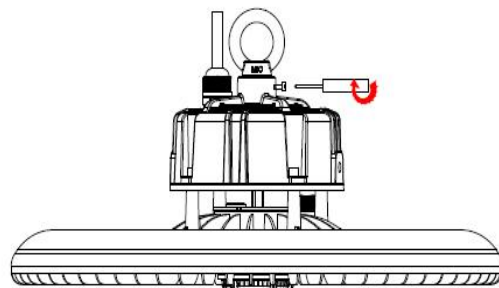
3. Attach the eyebolt to a secure structure.
