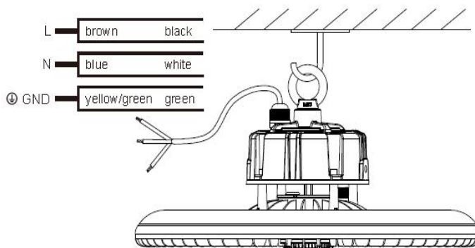
4. Connect the fixture input leads to the supply wire leads.
