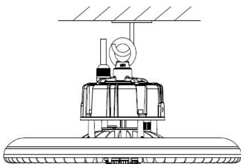
2. Secure the eyebolt with the locking screw.
